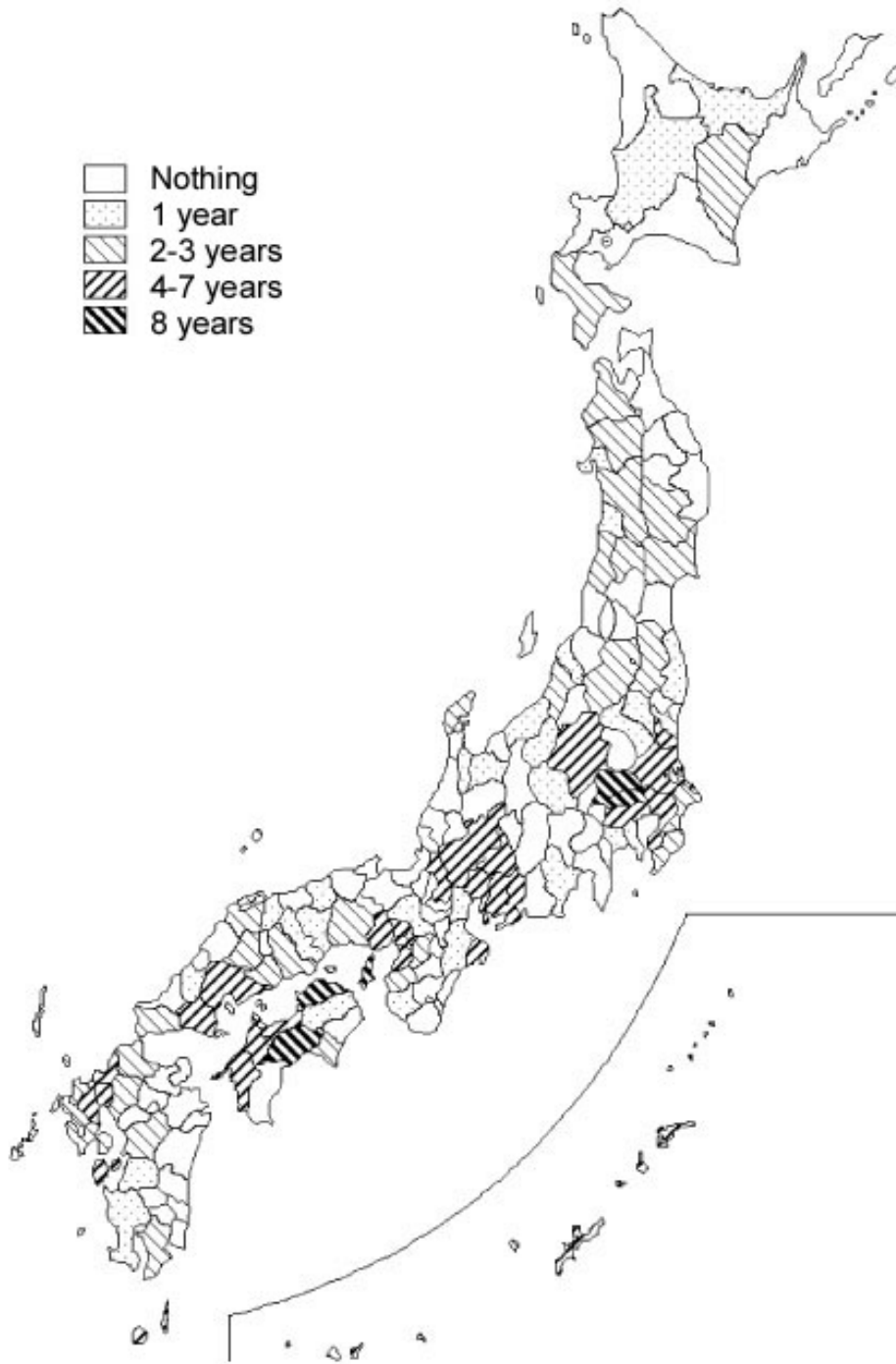
Fig. 6.5 Drought occurrence for a recent 20 years (MLIT, 2002).
