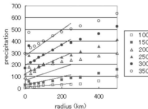
Fig. 6.11 Dependence of the radius of a scanning circle on the minimum areal precipitation. Figures in the legend indicate the duration of precipitation (days). Approximated lines based on a linear regression are also shown in the figure.
