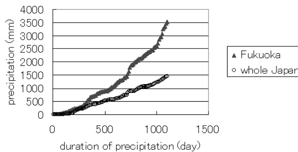
Fig. 6.6 Dependence of precipitation on the duration of precipitation.
