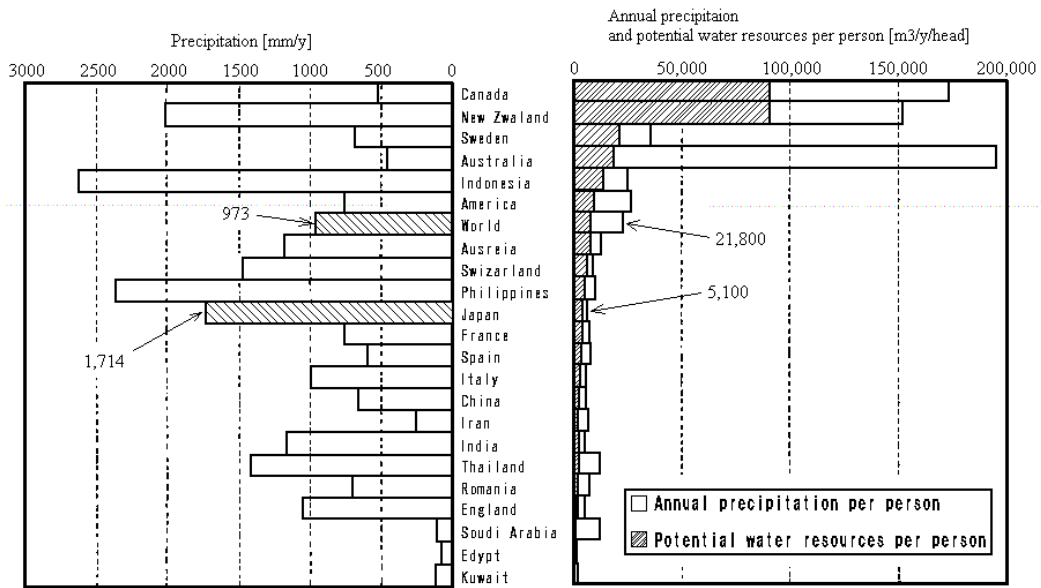
Fig. 6.1 Left: Annual precipitation. Right: Annual precipitation and potential water resources per person.
