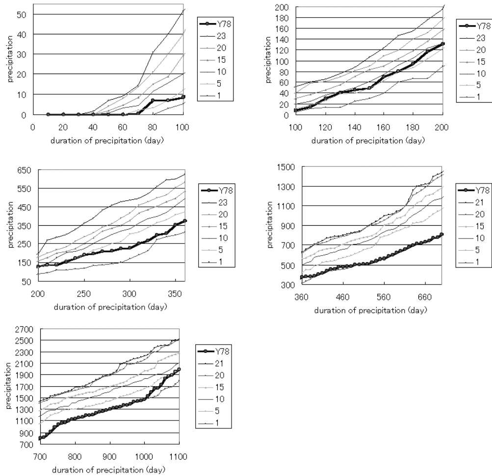
Fig. 6.9 Normalized precipitation vs the duration of precipitation (The seriousness of drought can be evaluated statistically using these figures. The relationship is divided into five sequences depending on the duration.)
