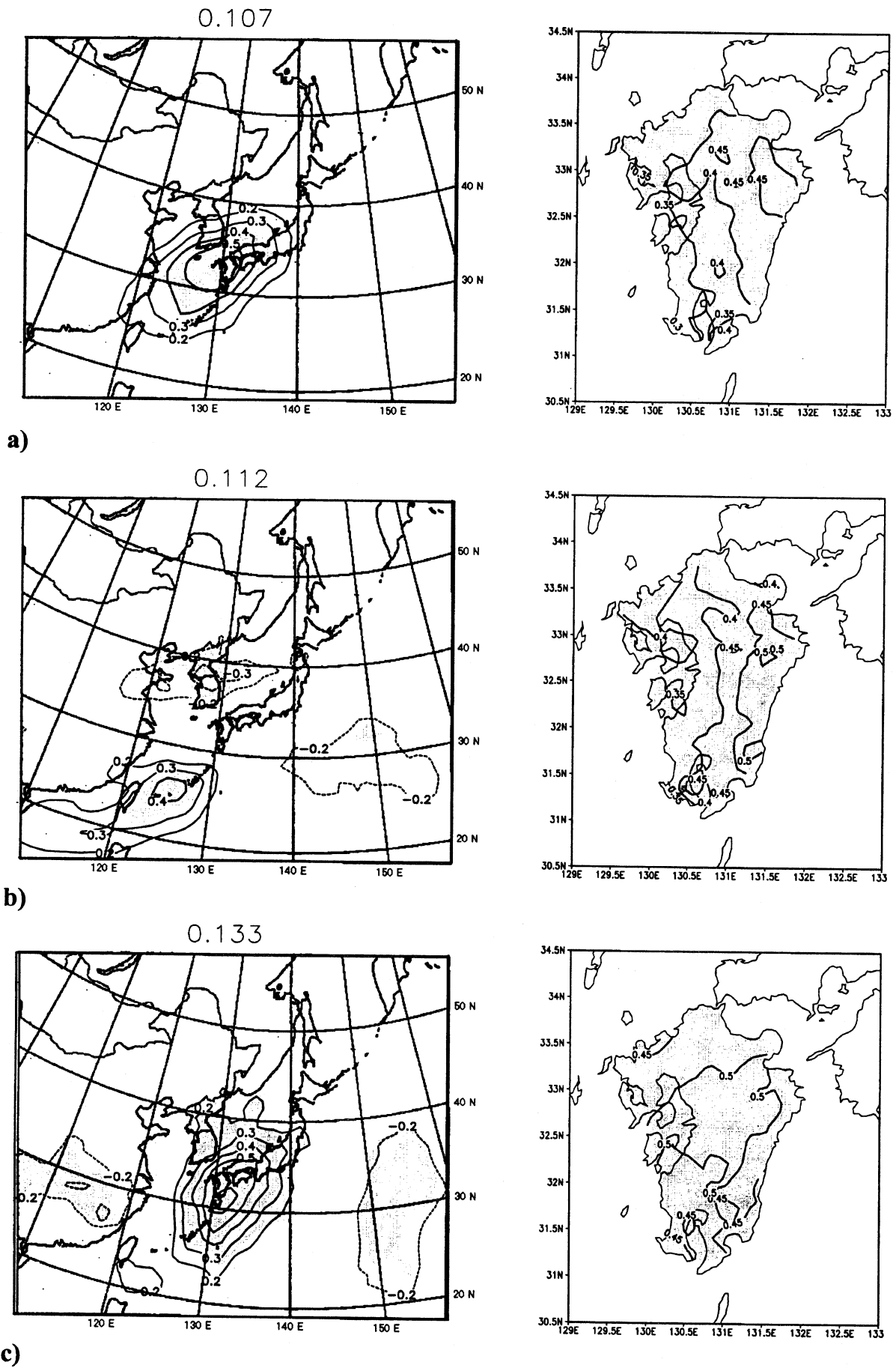
Fig. 4. Heterogeneous correlation maps between precipitation over Kyushu Island, and precipitable water (a), zonal winds at 850 hPa (b), and meridional winds at 850 hPa (c) for autumn. Lines and numbers as in Fig.3.
