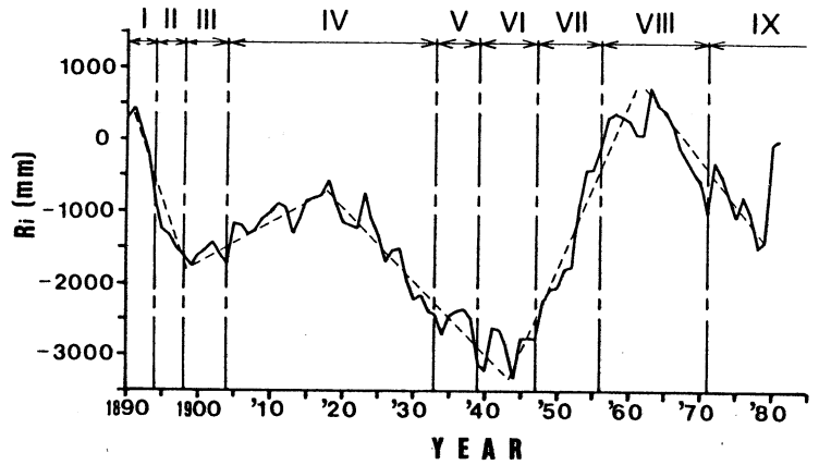
Fig.2 Plot of cumulation annual precipitation departures from mean. Broken line indicates the general tendency.
