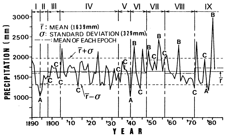
Fig.3 The annual precipitation sequence divided by AKF into nice different epochs. A, B and C are the types of the abnormal precipitation detected by OKF.
