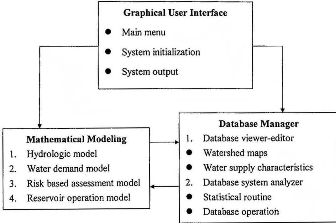
Fig. 3. Three main components of the proposed DSS
