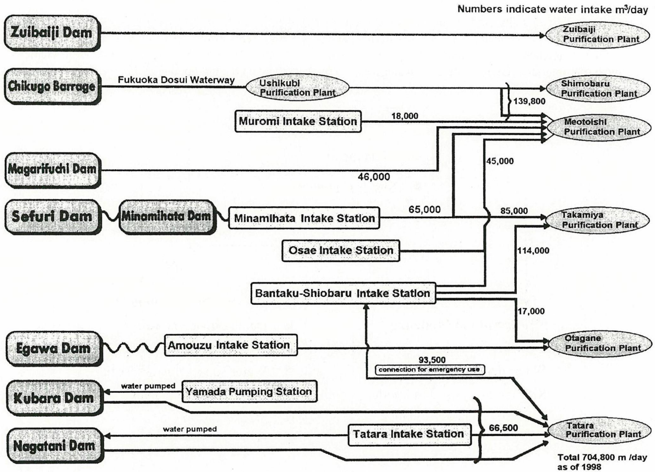
Fig. 2. Fukuoka City water supply network
