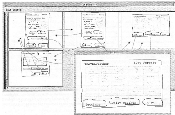
Figure 2.15: A sketch-based system that supports GUI designs (Landay and Myers 2001).
